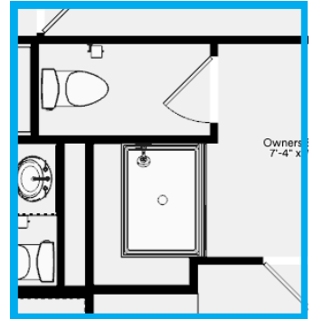
TILE SHOWER WALLS W/ SEAT
