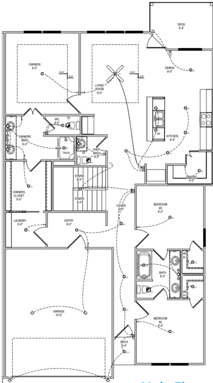
Main Floor
