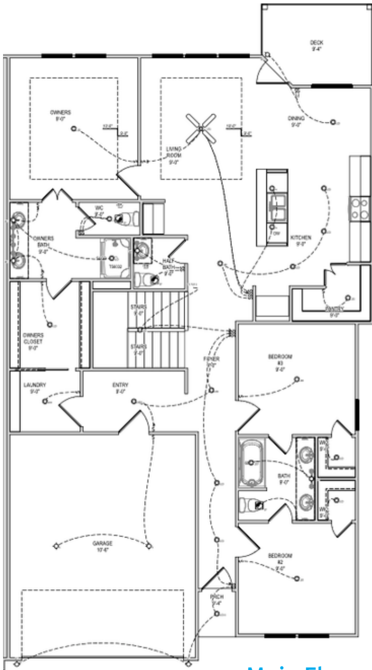
Main Floor
